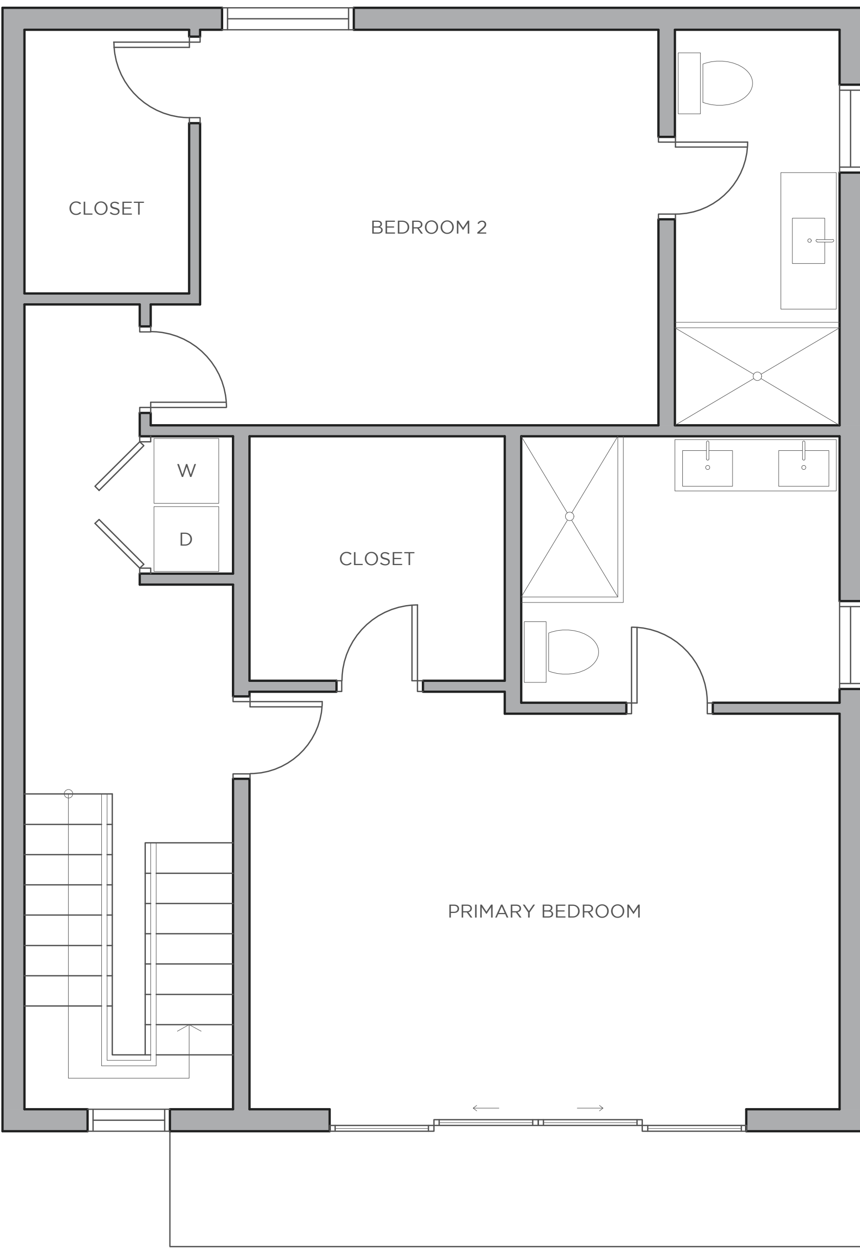
THIRD FLOOR
